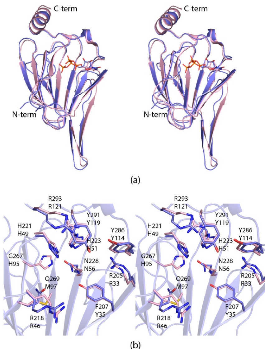
Figure 3. Comparison of the cupin domain of FdtD and the A. thermoaerophilus 3,4-ketoisomerase (PDB code 2PA7). A superposition of the ribbon drawings for the A. thermoaerophilus 3,4-ketoisomerase (pink) and the FdtD cupin domain (light blue) is shown in panel a. The bound dTDP ligands are drawn in stick representations. A close-up view of the two active sites, without the dTDP ligands, is displayed in panel b. The A. thermoaerophilus 3,4-ketoisomerase and the FdtD cupin domain are colored in pink and light blue, respectively. The labels on the top refer to those amino acids found in the cupin domain of FdtD, whereas those on the bottom correspond to residues in the A. thermoaerophilus 3,4-ketoisomerase.
