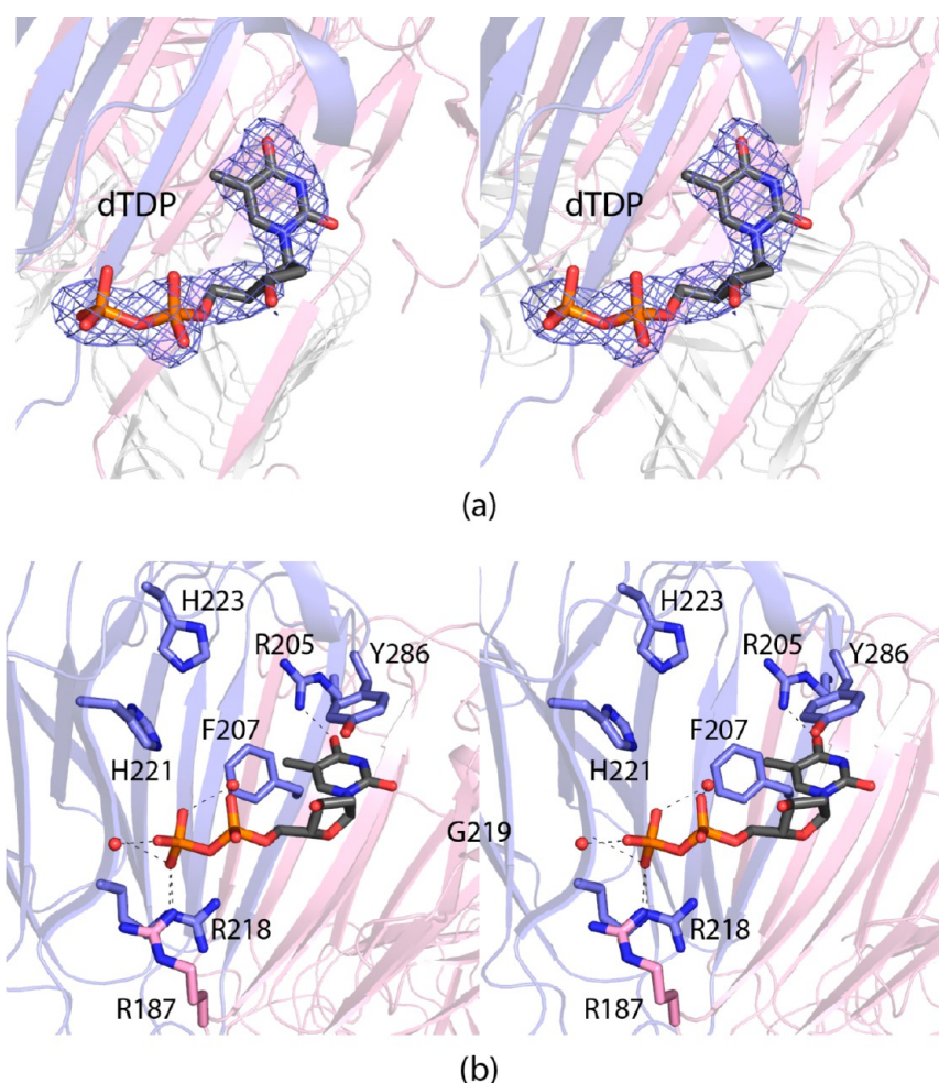
Figure 2. Active site of the FdtD cupin domain. Electron density corresponding to the bound dTDP is presented in panel a. The omit map, contoured at 2\sigma , was calculated at 2.2 Å resolution with coefficients of the form F_o - F_c , where F_o was the native structure factor amplitude, and F_c was the calculated structure factor amplitude (the ligand was not included in the X-ray coordinate file, so it did not contribute to the phasing). A close-up view of the region surrounding the dTDP ligand is shown in panel b. The dashed lines indicate potential hydrogen bonds. Ordered water molecules are represented by small red spheres. Arg 187, highlighted in pink bonds, is contributed by the second subunit in the dimer as a result of domain swapping.
