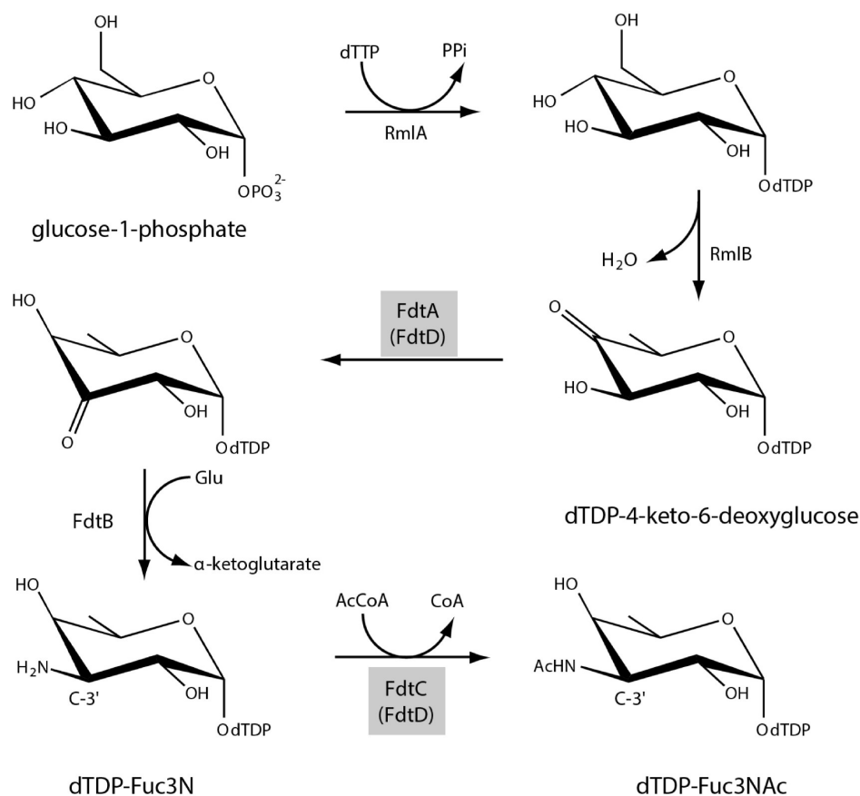
Scheme 1. Biosynthetic Pathway for the Production of dTDP-Fuc3NAc
