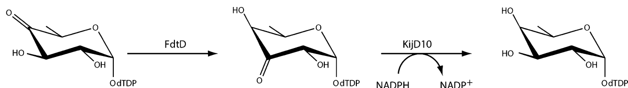
Scheme 3. Pathway Used to Determine Kinetic Constants for the 3,4-Ketoisomerase Activity
