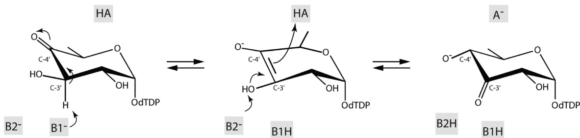
Scheme 5. Possible Catalytic Mechanism for a 3,4-Ketoisomerase
