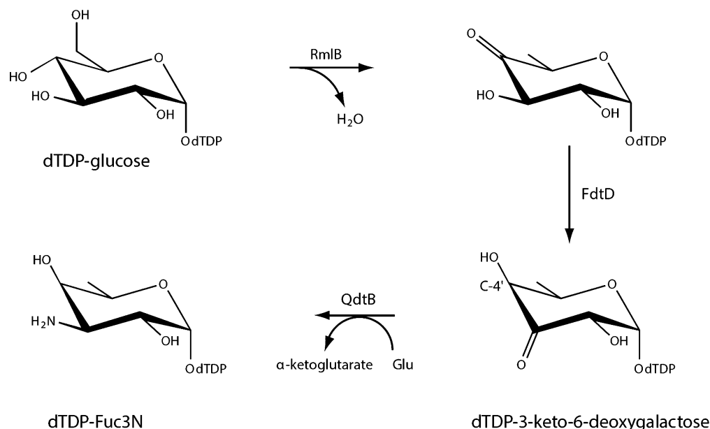
Scheme 2. Pathway to Verify 3,4-Ketoisomerase Activity
