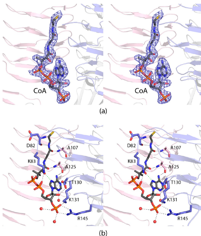
Figure 5. Binding of CoA to the \beta -helix domain of FdtD. Electron density corresponding to bound CoA is shown in panel a. The map was calculated as described in the legend to Figure 2 and contoured at 2\sigma . A close-up view of the CoA binding pocket is displayed in panel b. The CoA is highlighted in gray and orange bonds. Those residues belonging to subunits 1 and 2 are colored in blue and pink, respectively. Ordered water molecules are drawn as red spheres. The dashed lines indicate possible hydrogen bonding interactions between the cofactor and the protein.
