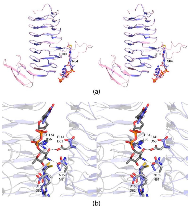
Figure 6. Comparison of the FdtD N-acetyltransferase domain with the N-acetyltransferases from B. petrii (PDB code 3MQH) and T. thermosaccharolyticum (3FSC). The structure of the \beta -helix domain of FdtD most closely resembles that of the enzyme from B. petrii . A superposition of the ribbon drawings for FdtD (blue) and the B. petrii enzyme (pink) is presented in panel a. The B. petrii enzyme is larger with a globular domain following the \beta -helix motif. In both enzymes, the regularity of the \beta -helix is broken by an extended loop, which is ordered in the B. petrii enzyme but disordered in the FdtD model. The conformation of the acetyl-CoA ligand, when bound to the B. petrii enzyme, matches that observed for CoA when complexed to FdtD. Shown in panel b is a superposition of the active site of the T. thermosaccharolyticum N-acetyltransferase with bound dTDP-Fuc3N (gray) onto the FdtD active site (blue). The dashed lines indicate hydrogen bonds that occur between the T. thermosaccharolyticum N-acetyltransferase and dTDP-Fuc3N. The residues in the T. thermosaccharolyticum enzyme responsible for anchoring the sugar into the active site include His 134, Glu 141, Asn 159, and Asp 160. These residues correspond to Lys 56, Asp 63, Asn 81, and Asp 82 in FdtD. Mutations of these residues in the T. thermosaccharolyticum enzyme did not result in loss of enzymatic activity.
