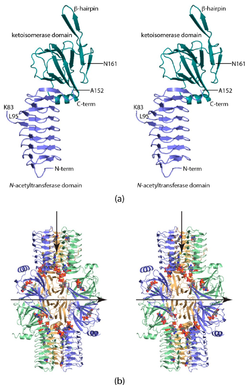
Figure 1. Structure of FdtD. A ribbon representation of one subunit of FdtD is shown in panel a. The N-terminal and C-terminal domains, which contain the catalytic residues responsible for the N -acetyltransferase and 3,4-ketoisomerase activities of FdtD, are displayed in light blue and teal, respectively. A complete FdtD hexamer is depicted in panel b. The dTDP and CoA ligands are shown in space-filling representations. The view in panel b is looking down a 2-fold rotational axis that relates one trimer to another within the hexamer. Thus, the subunit colored in green in one trimer is related by a rotation of 180° to the subunit drawn in green in the second trimer. The FdtD hexamer displays 322 symmetry. The second 2-fold lies in the plane of the paper and is indicated by the horizontal arrow. The 3-fold axis also lies in the plane of the paper and is indicated by the vertical arrow. All figures were created using PyMOL. 30
